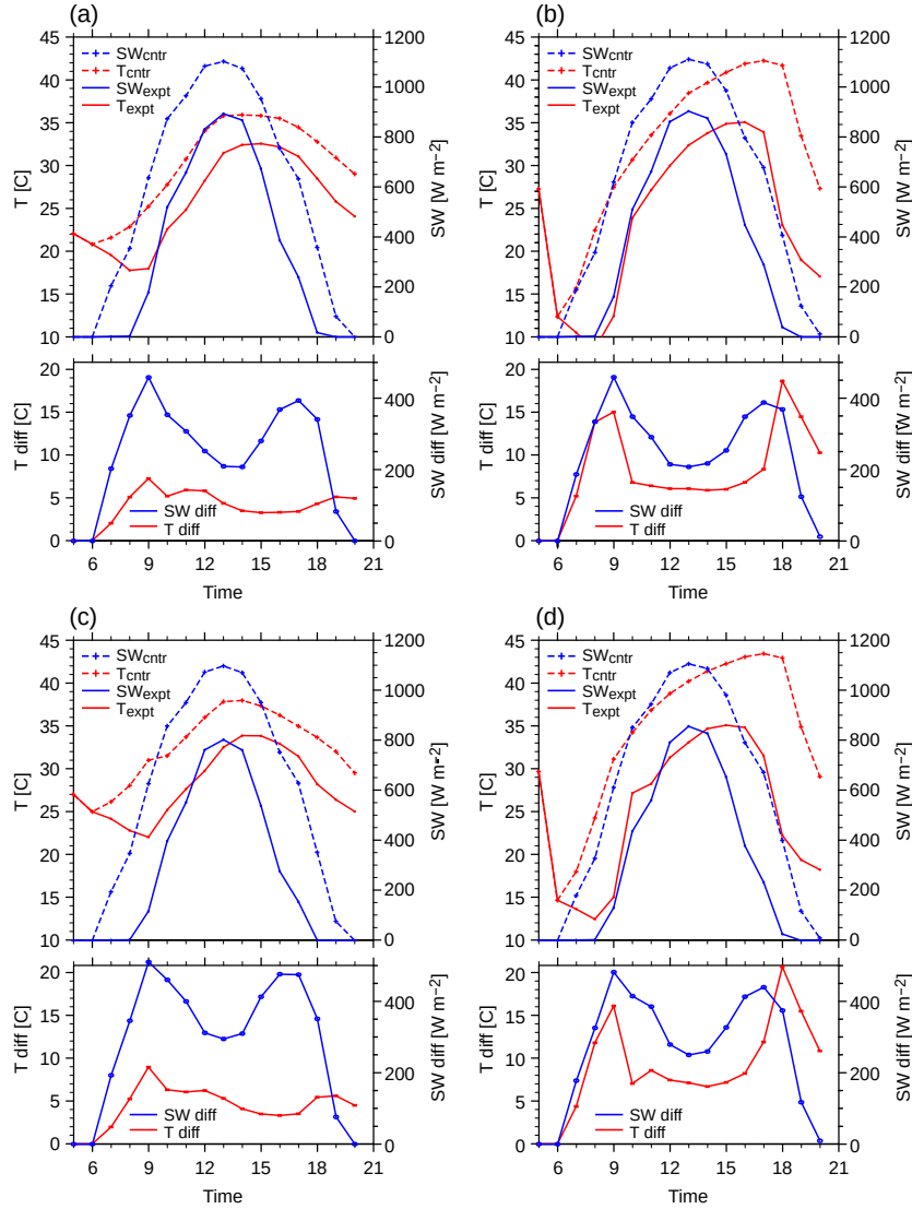
Fig. 10. Time-series (local time) of surface air temperature [°C] (red) and surface shortwave flux [ W m^{-2} ] (blue); the upper panel shows the control run and experimental surface air temperature and surface shortwave radiation flux, and the lower panel shows the differences between the control run and the experimental surface air temperature and surface shortwave radiation flux for (a) Los Angeles, July 22nd, (b) Central Valley (Fresno), July 22nd, (c) Los Angeles, July 23rd, (d) Central Valley (Fresno), July 23rd.
