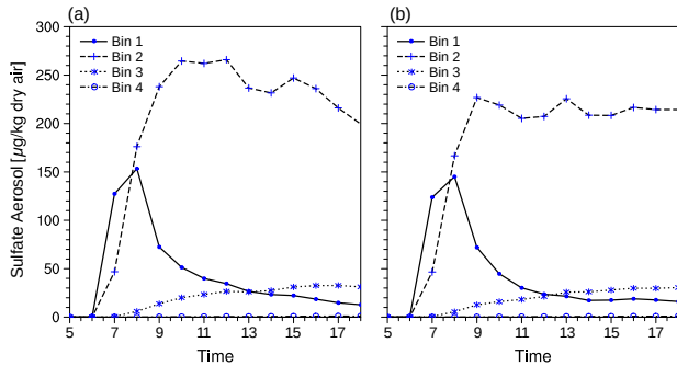
Fig. 9. Sulfate aerosol concentrations [ \mu\text{g kg}^{-1} dry air] time-series (local time) at the level of the injection for July 22nd for a point location (a) in Los Angeles and (b) in the Central Valley (Fresno). See Fig. 1 for point locations.
