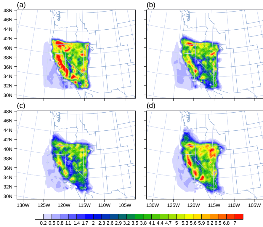
Fig. 8. Surface air temperature differences, [ ^{\circ}\text{C} ] between large-scale 30\mu\text{g m}^{-2} \text{ s}^{-1} experiment and the control in July 23rd at hours (a) 10:00 LT, (b) 12:00 LT, (c) 14:00 LT, and (d) 16:00 LT.
